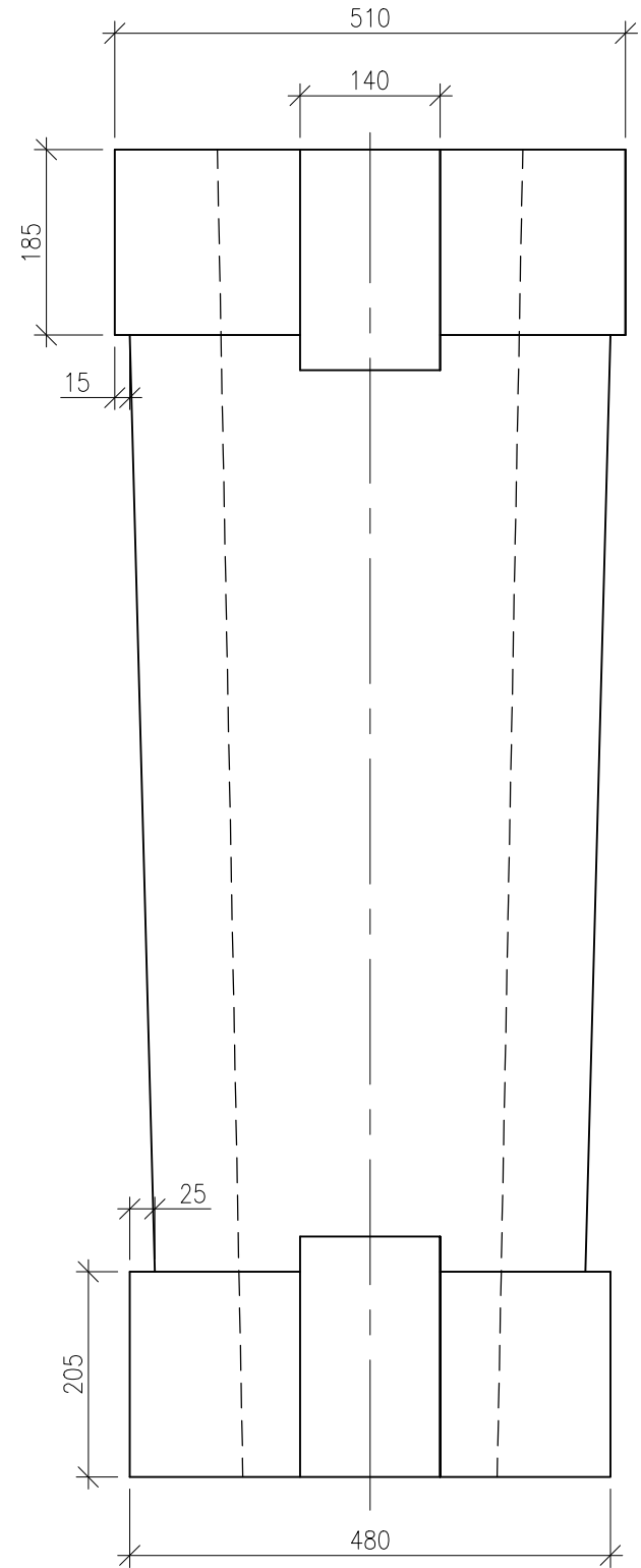
SIDE VIEW
