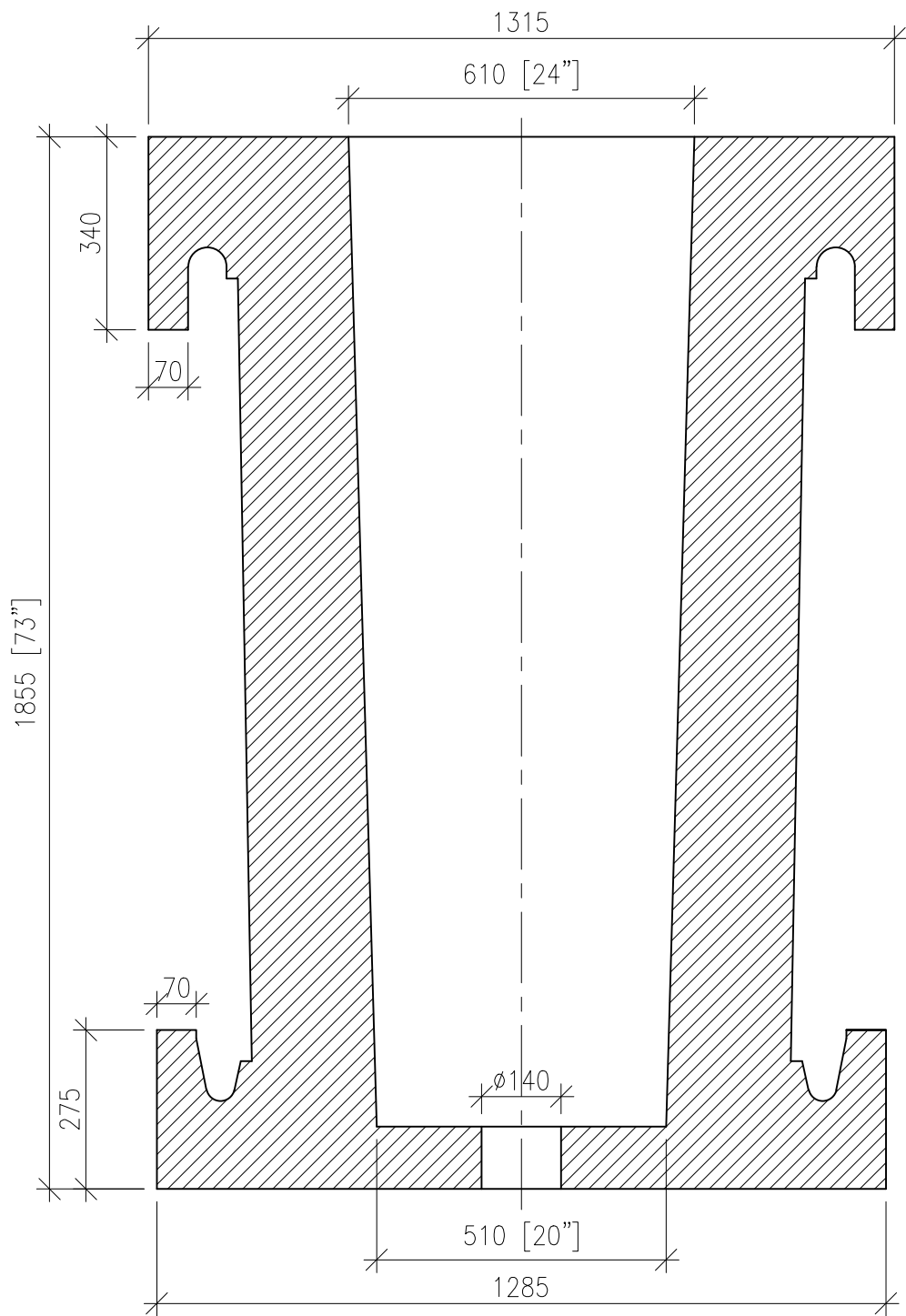
ELEVATION SECTION - AA
