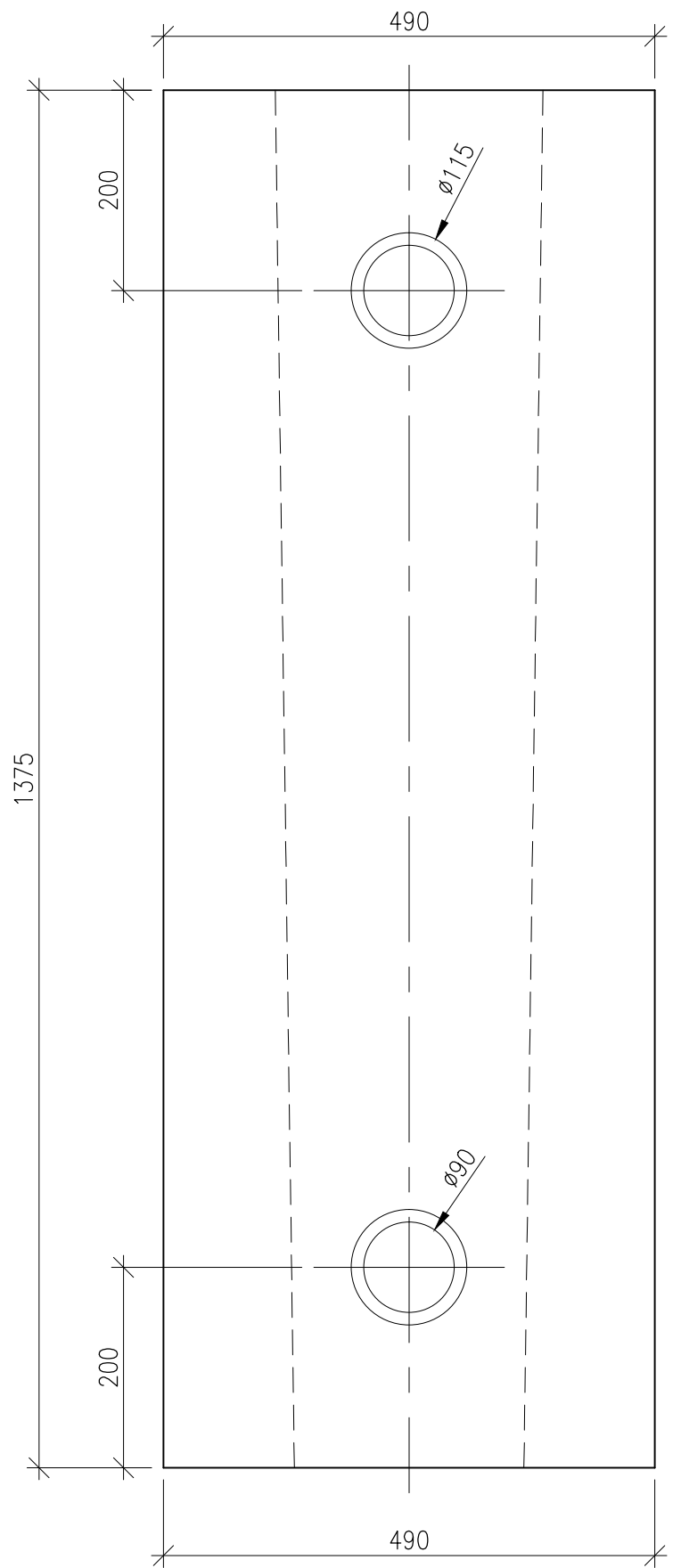
SIDE VIEW
