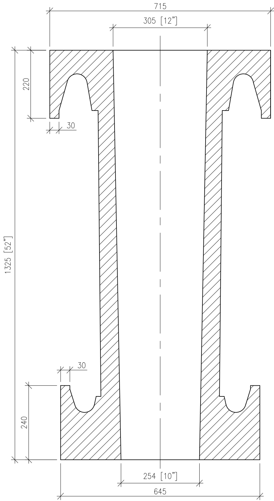
ELEVATION SECTION - AA
