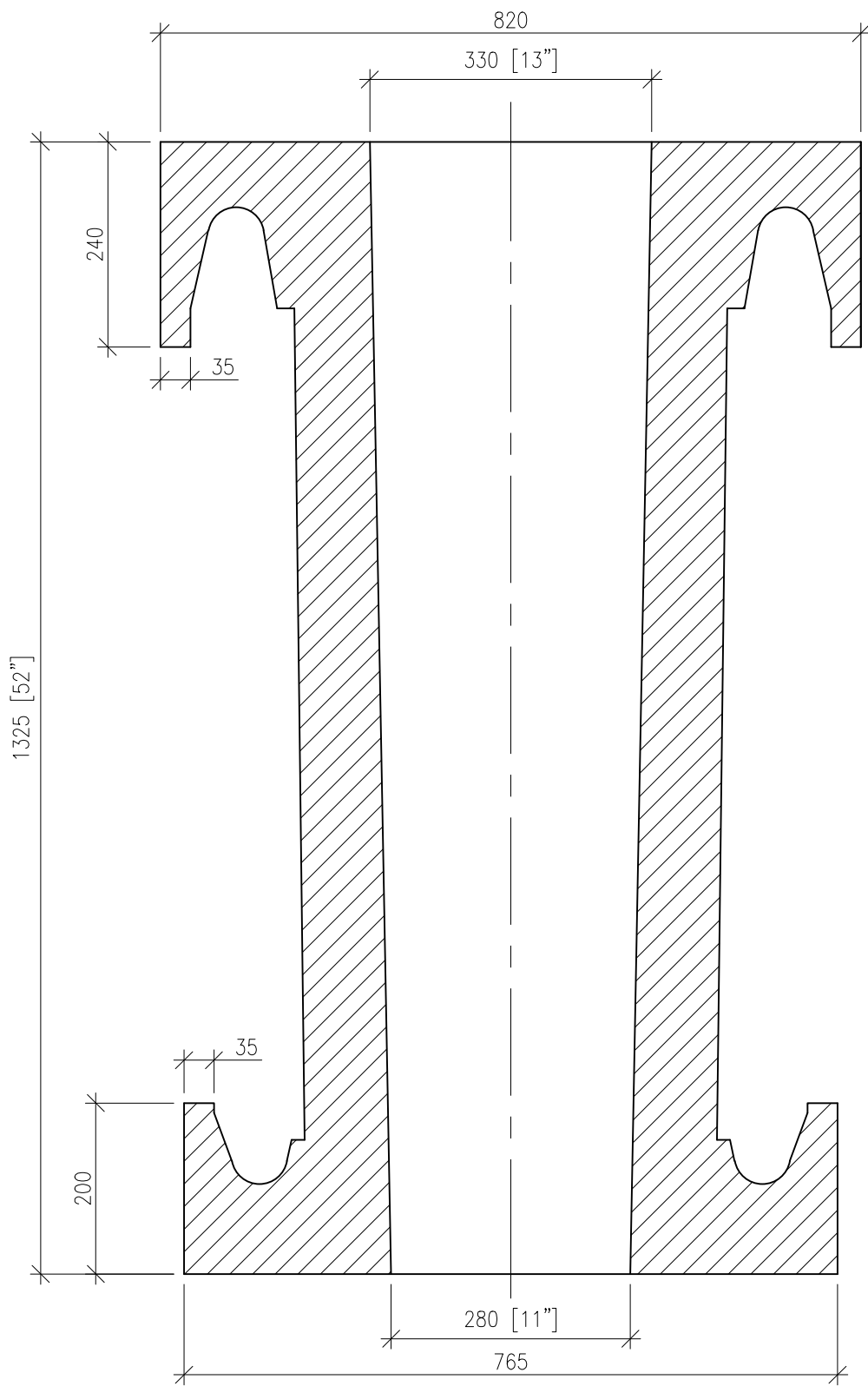
ELEVATION SECTION - AA
