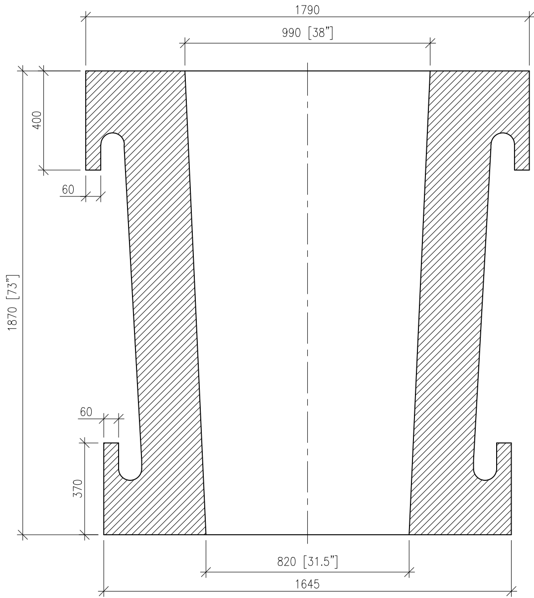
ELEVATION SECTION - AA
