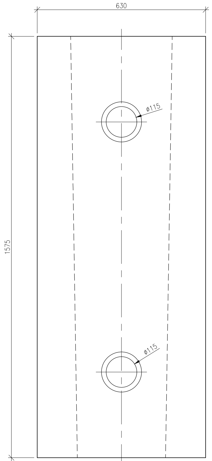
SIDE VIEW
