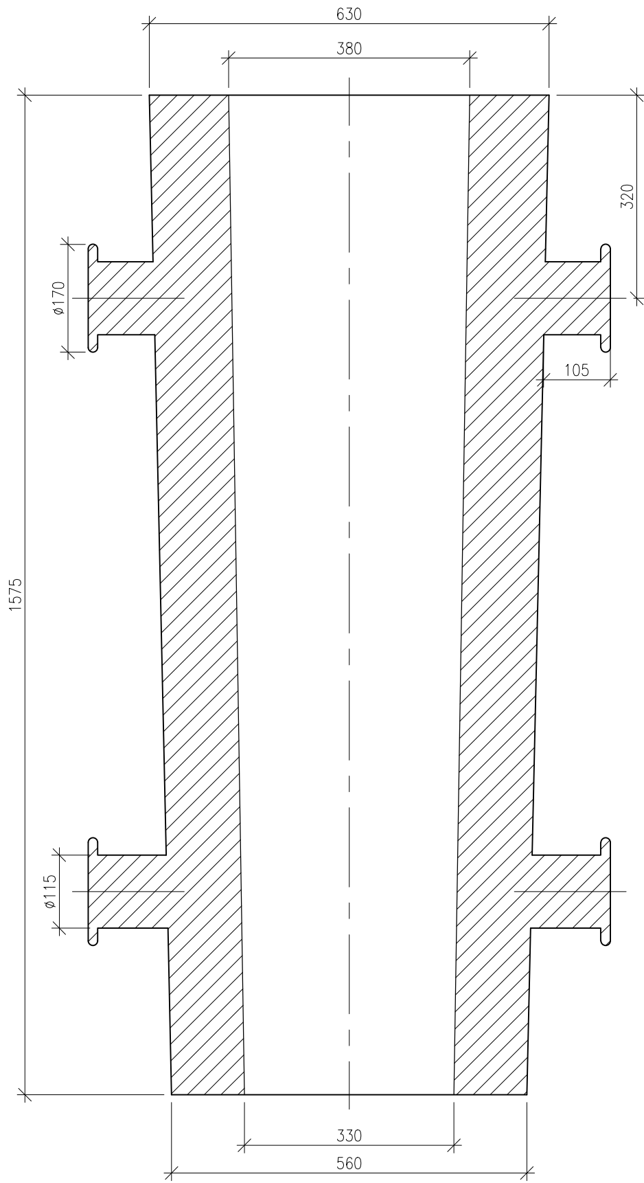
ELEVATION SECTION - AA
