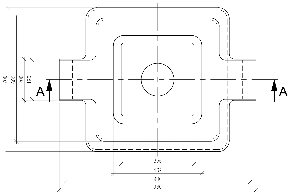
TOP VIEW
