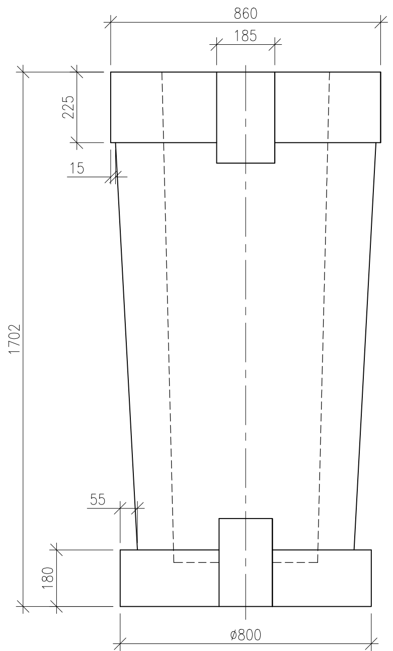
SIDE VIEW
