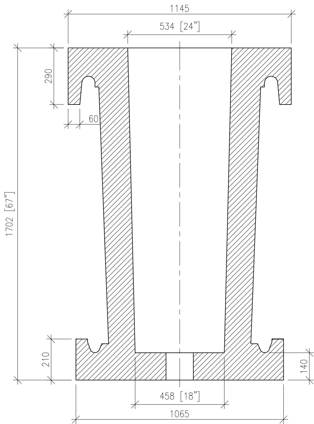
ELEVATION SECTION - AA
